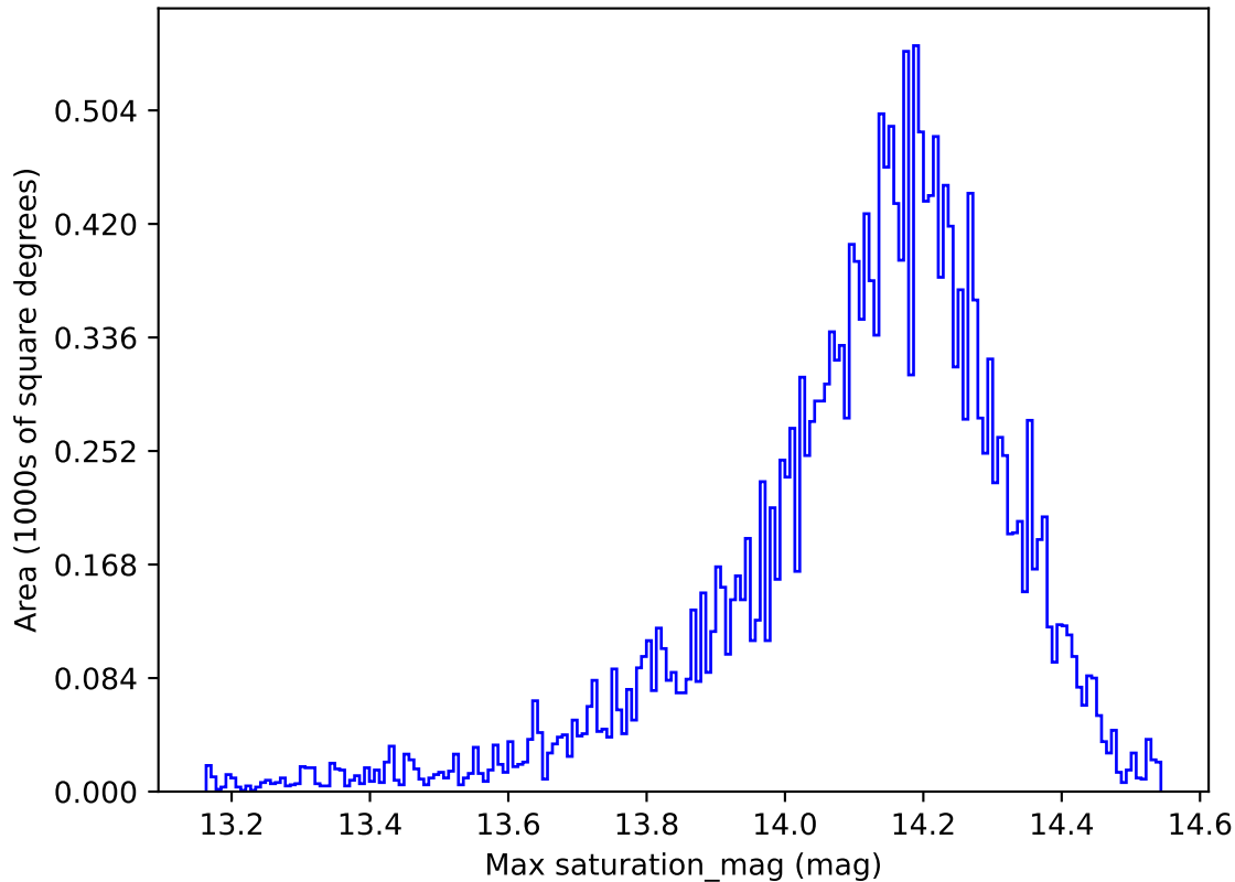
too_elab_r8_d2_gz_v3.4_10yrs All sky y band: Max saturation_mag
