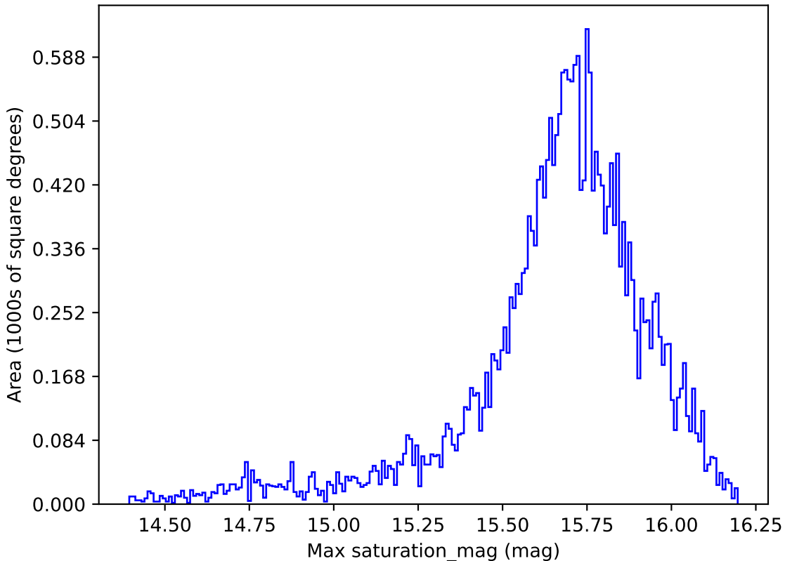
too_elab_r8_d2_gz_v3.4_10yrs All sky r band: Max saturation_mag
