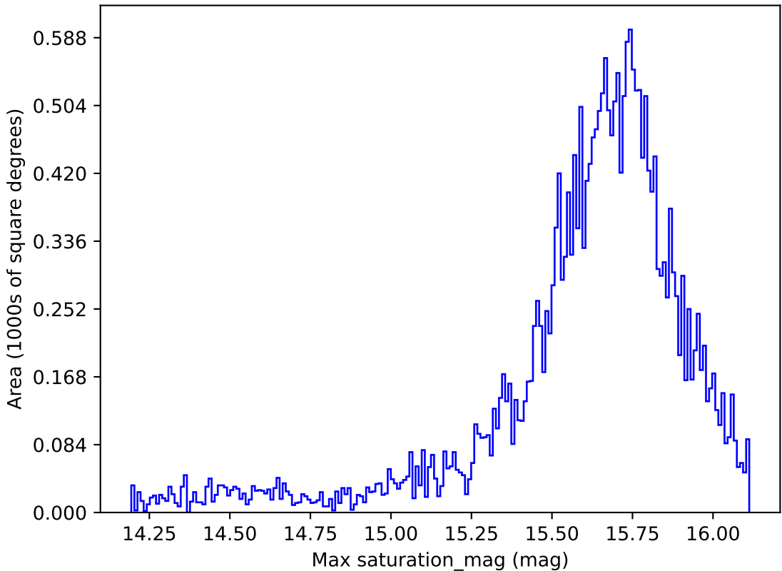
too_elab_r8_d2_gz_v3.4_10yrs All sky g band: Max saturation_mag
