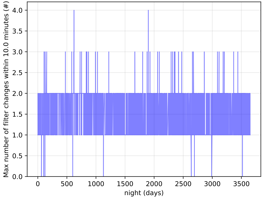
too_elab_r8_d2_gz_v3.4_10yrs Per Night: Max number of filter changes within 10.0 minutes
