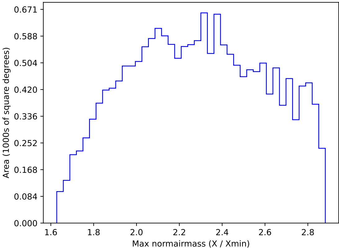
too_elab_r8_d2_gz_v3.4_10yrs WFD z band: Max normairmass
