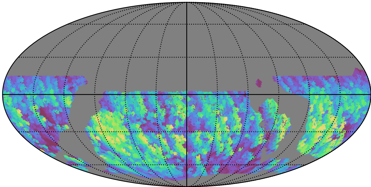
too_elab_r8_d2_gz_v3.4_10yrs WFD y band: Max normairmass
