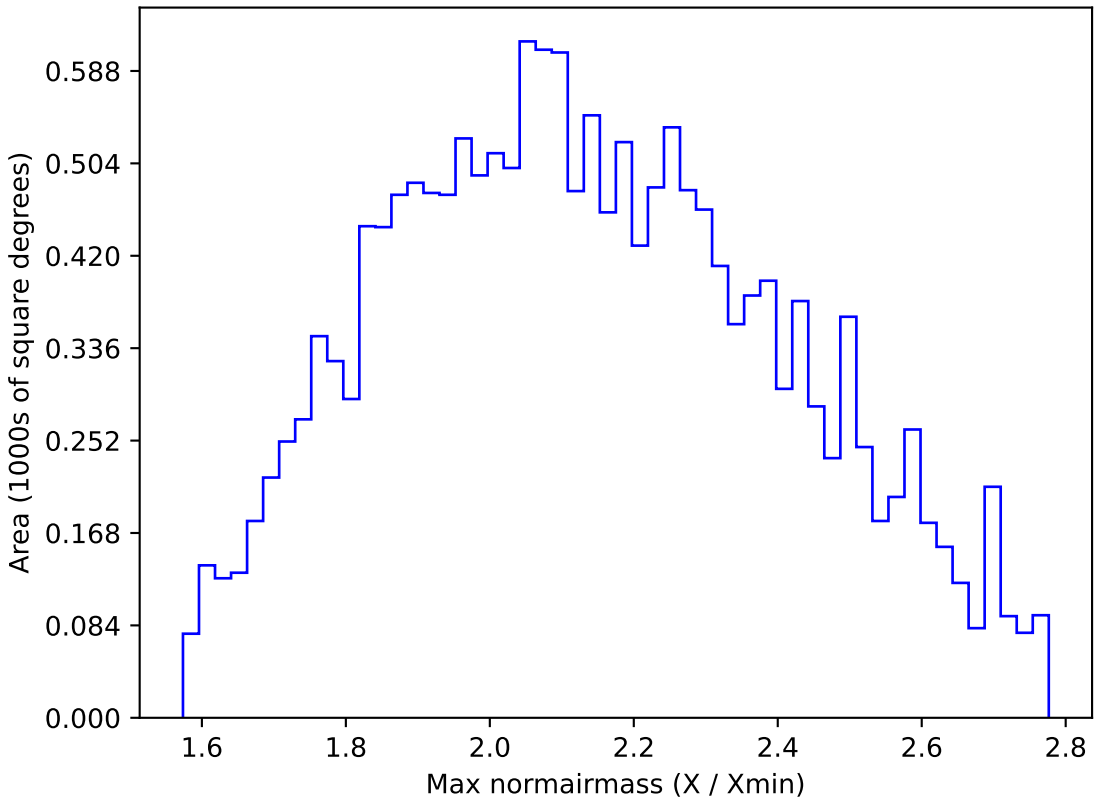
too_elab_r8_d2_gz_v3.4_10yrs WFD y band: Max normairmass
