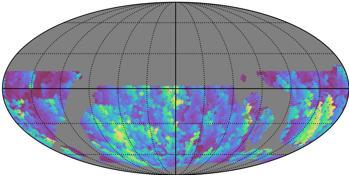
too_elab_r8_d2_gz_v3.4_10yrs WFD u band: Max normairmass
