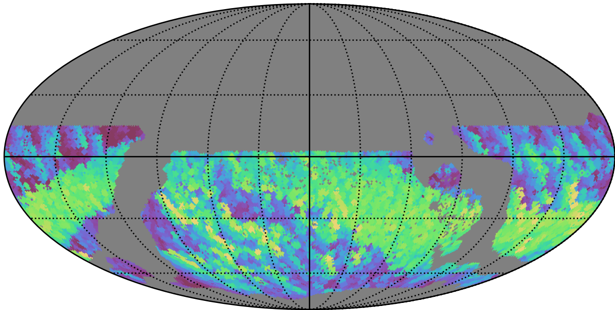
too_elab_r8_d2_gz_v3.4_10yrs WFD r band: Max normairmass
