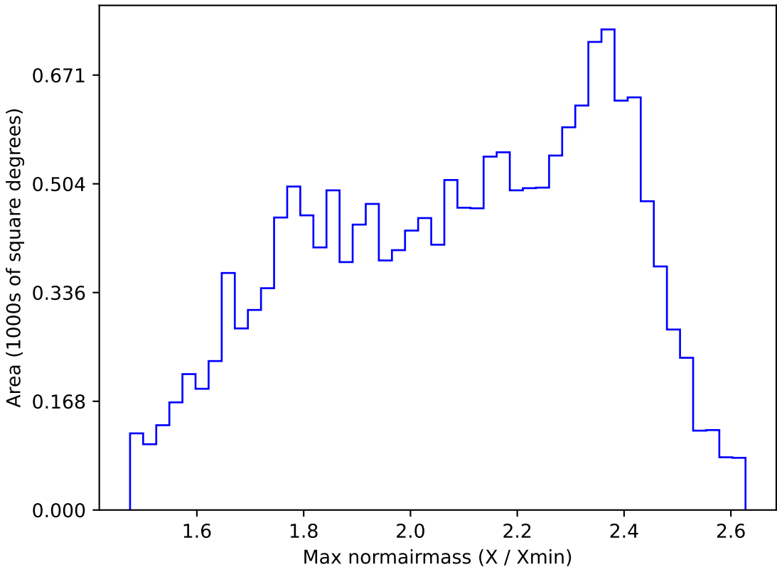
too_elab_r8_d2_gz_v3.4_10yrs WFD r band: Max normairmass
