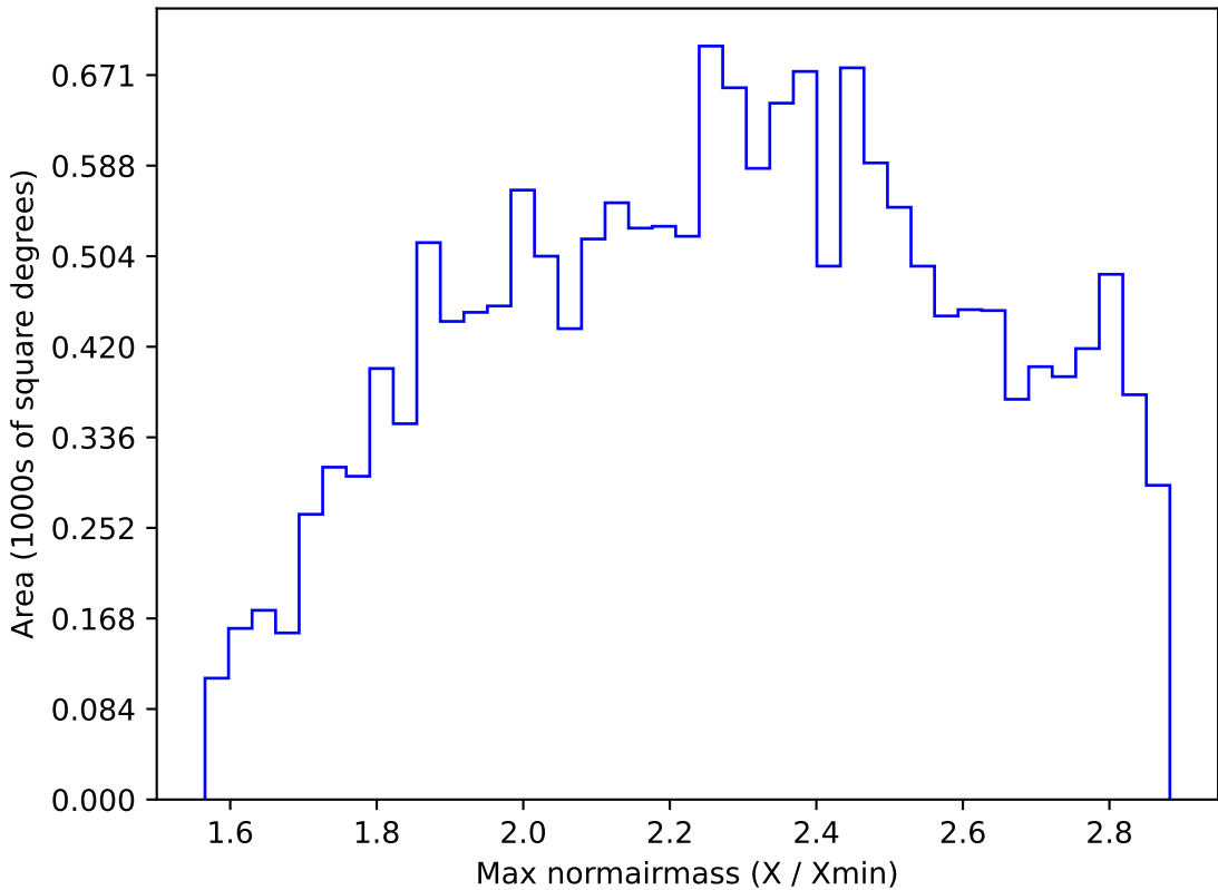
too_elab_r8_d2_gz_v3.4_10yrs WFD i band: Max normairmass
