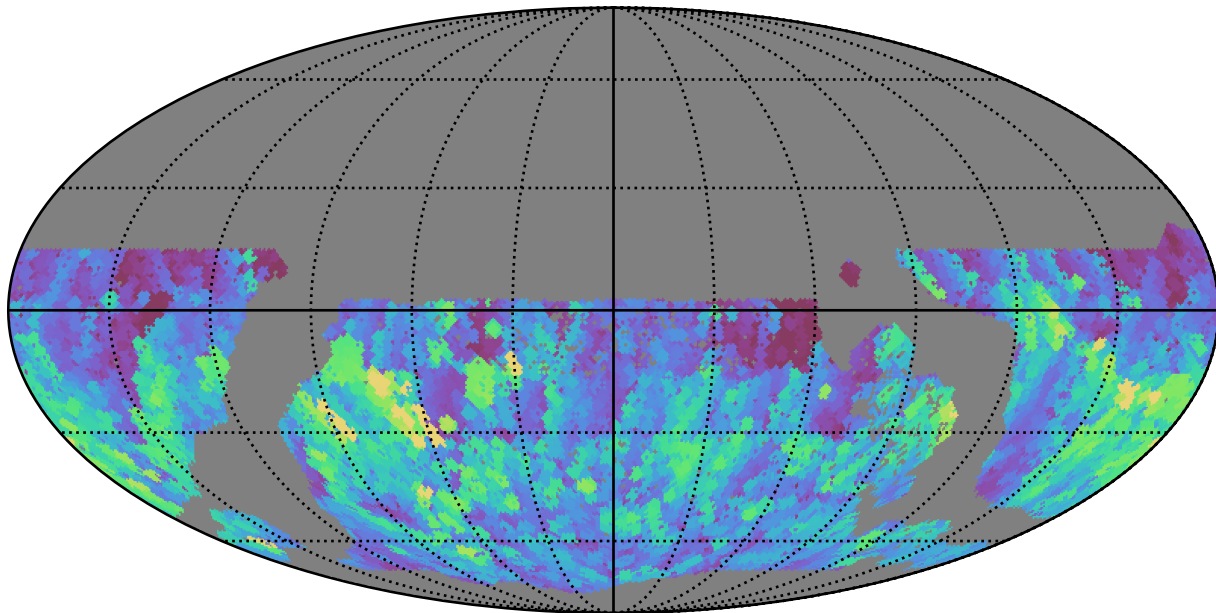
too_elab_r8_d2_gz_v3.4_10yrs WFD g band: Max normairmass
