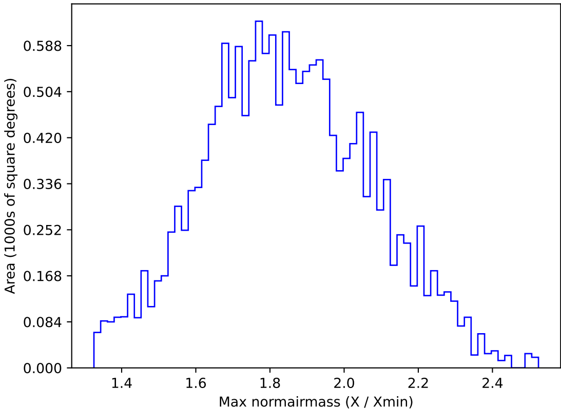
too_elab_r8_d2_gz_v3.4_10yrs WFD g band: Max normairmass
