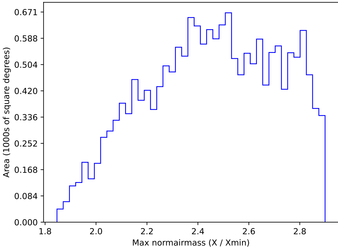
too_elab_r8_d2_gz_v3.4_10yrs WFD all bands: Max normairmass
