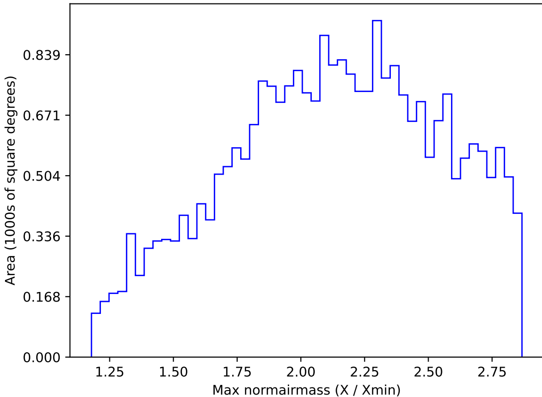
too_elab_r8_d2_gz_v3.4_10yrs All sky z band: Max normairmass
