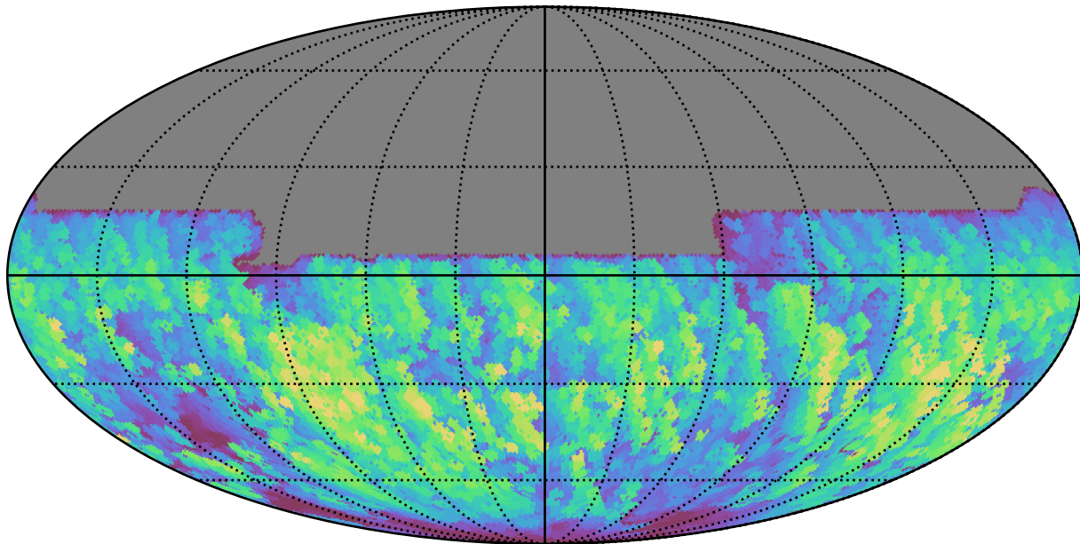
too_elab_r8_d2_gz_v3.4_10yrs All sky y band: Max normairmass
