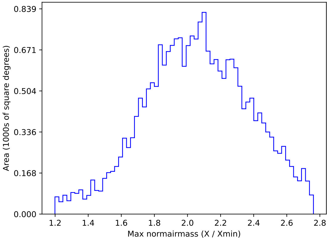
too_elab_r8_d2_gz_v3.4_10yrs All sky y band: Max normairmass
