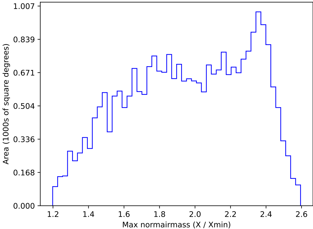
too_elab_r8_d2_gz_v3.4_10yrs All sky r band: Max normairmass
