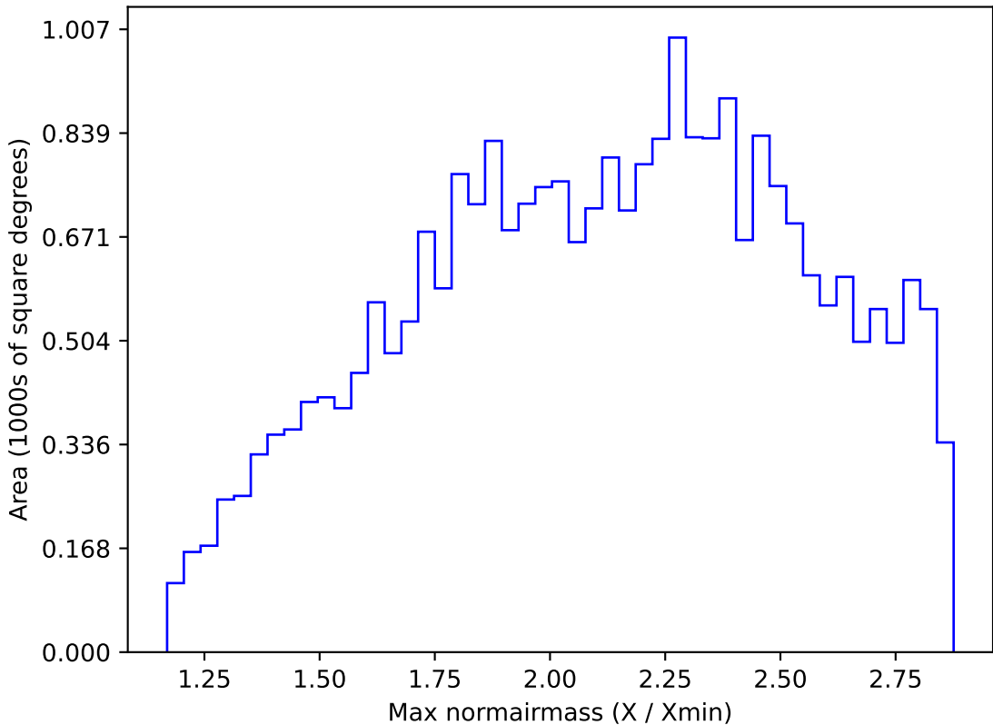
too_elab_r8_d2_gz_v3.4_10yrs All sky i band: Max normairmass
