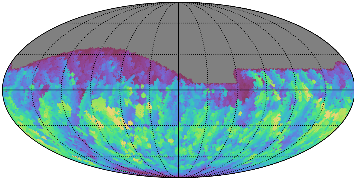
too_elab_r8_d2_gz_v3.4_10yrs All sky g band: Max normairmass
