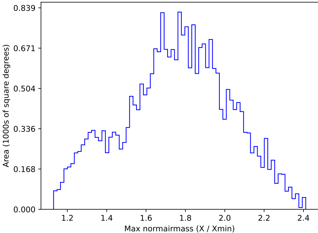
too_elab_r8_d2_gz_v3.4_10yrs All sky g band: Max normairmass
