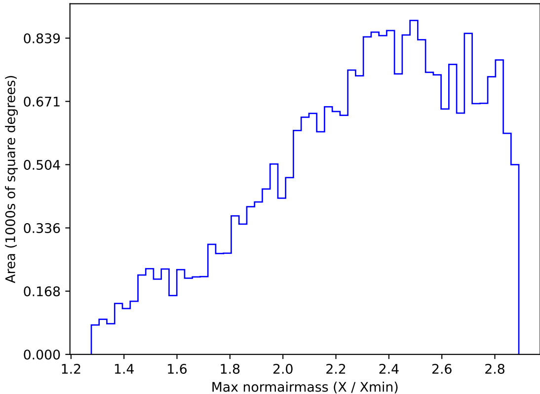
too_elab_r8_d2_gz_v3.4_10yrs All sky all bands: Max normairmass
