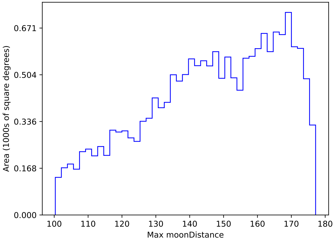
too_elab_r8_d2_gz_v3.4_10yrs WFD y band: Max moonDistance
