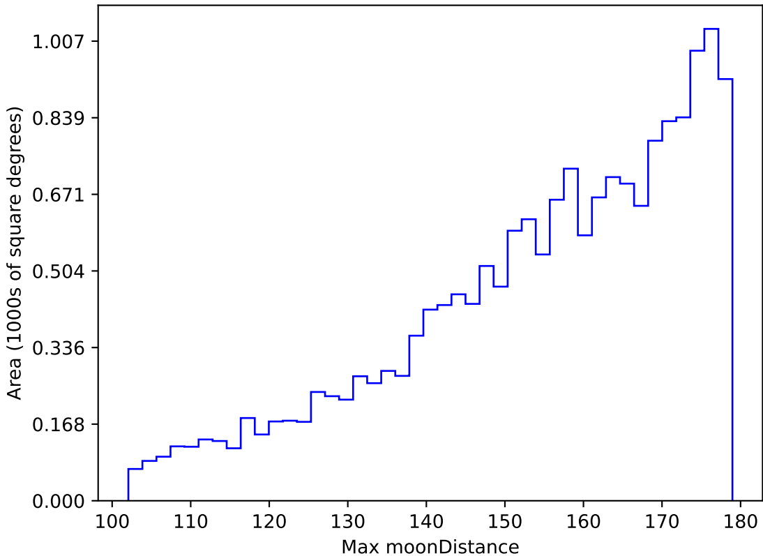
too_elab_r8_d2_gz_v3.4_10yrs WFD u band: Max moonDistance
