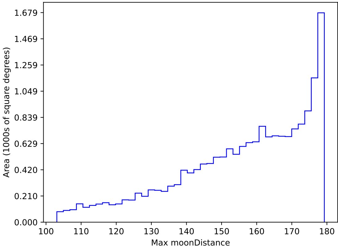
too_elab_r8_d2_gz_v3.4_10yrs WFD r band: Max moonDistance
