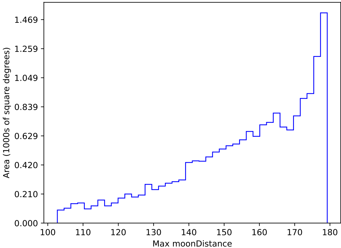
too_elab_r8_d2_gz_v3.4_10yrs WFD i band: Max moonDistance
