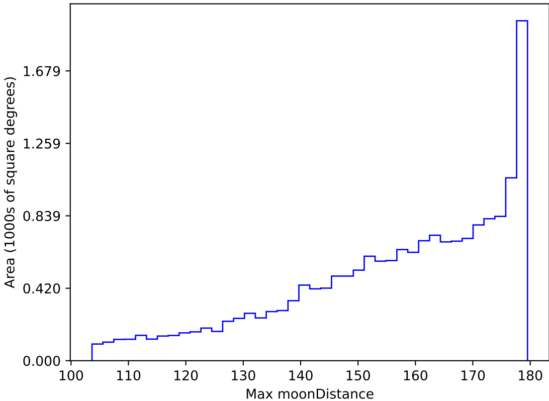
too_elab_r8_d2_gz_v3.4_10yrs WFD all bands: Max moonDistance
