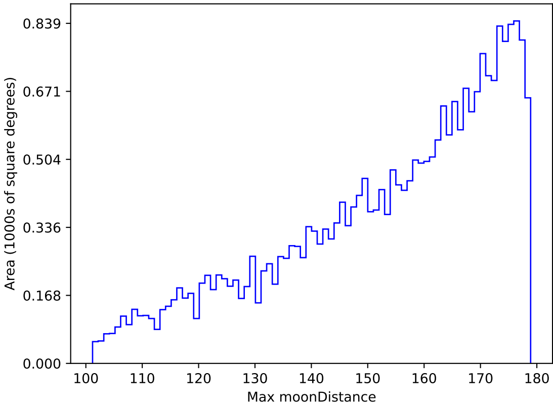
too_elab_r8_d2_gz_v3.4_10yrs All sky z band: Max moonDistance
