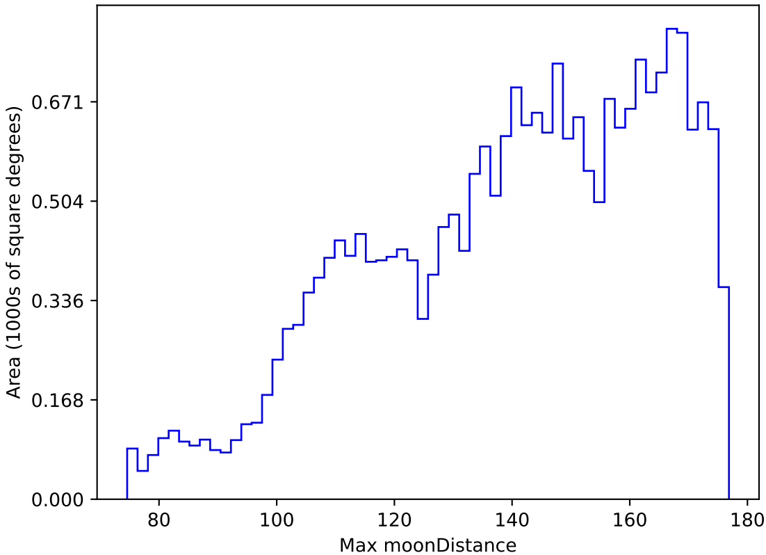
too_elab_r8_d2_gz_v3.4_10yrs All sky y band: Max moonDistance
