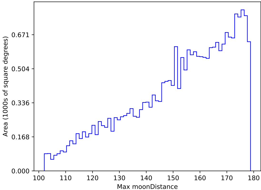
too_elab_r8_d2_gz_v3.4_10yrs All sky u band: Max moonDistance
