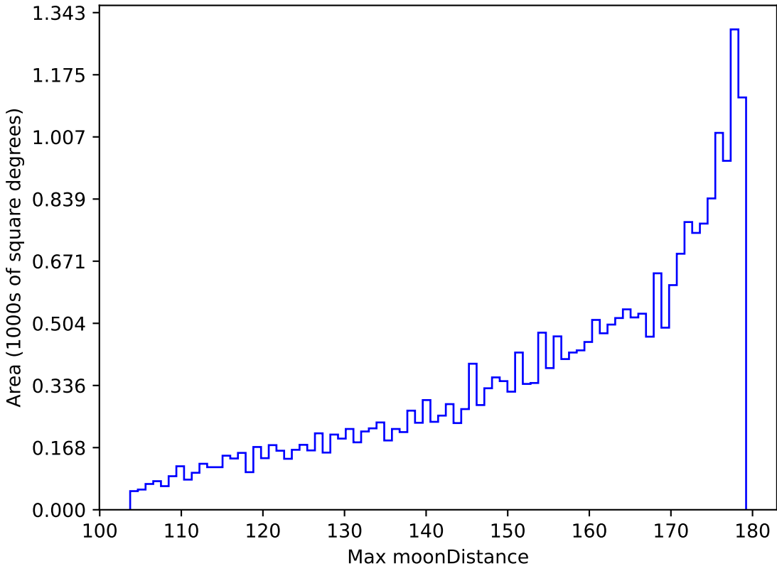
too_elab_r8_d2_gz_v3.4_10yrs All sky r band: Max moonDistance
