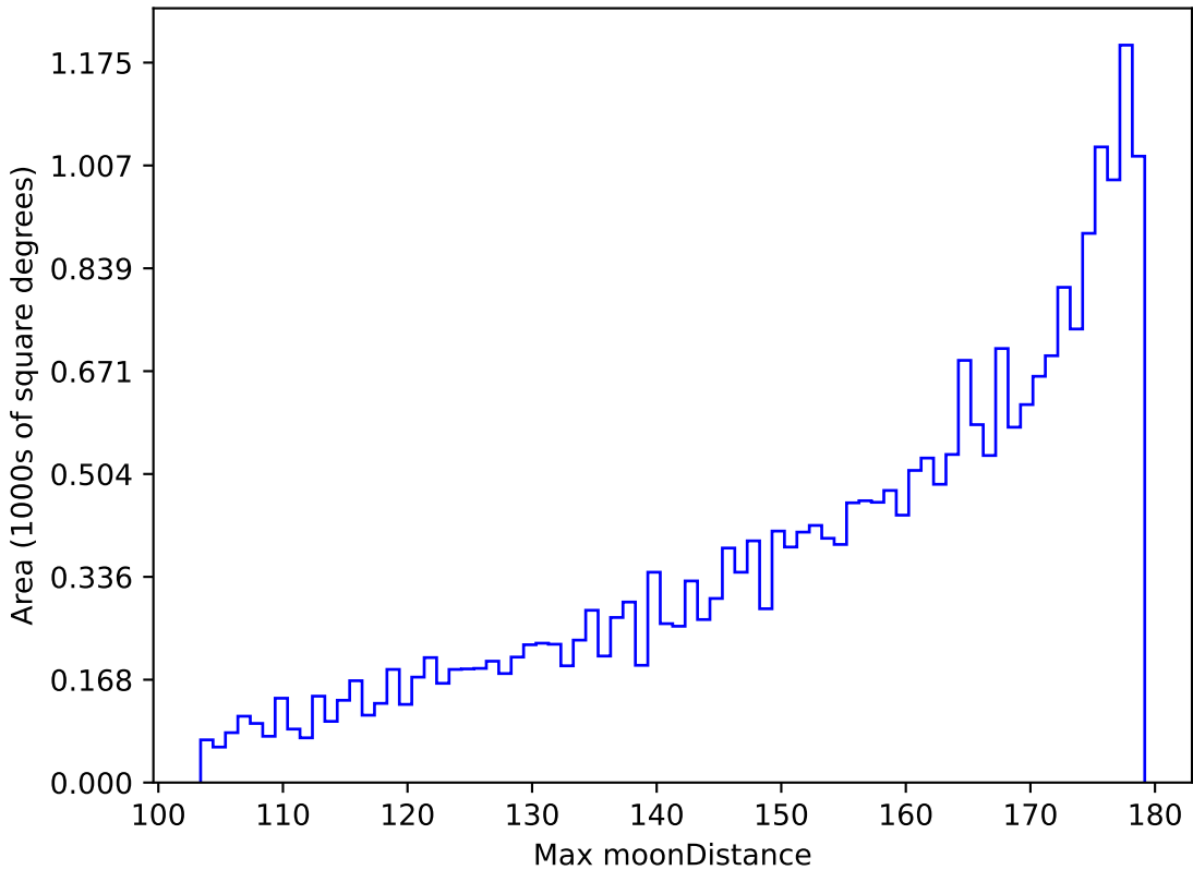
too_elab_r8_d2_gz_v3.4_10yrs All sky i band: Max moonDistance
