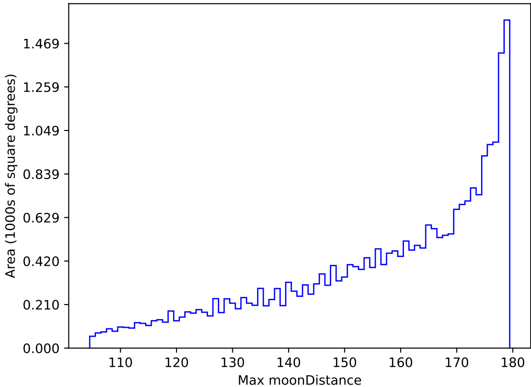
too_elab_r8_d2_gz_v3.4_10yrs All sky all bands: Max moonDistance
