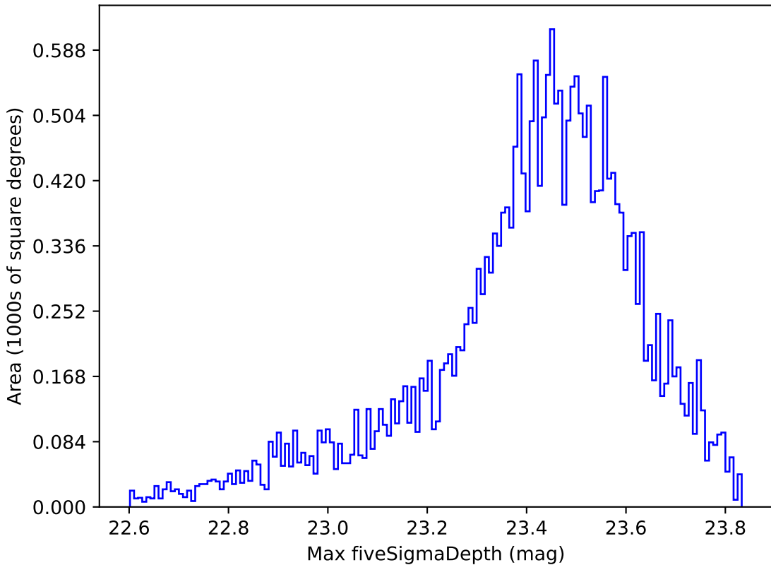
too_elab_r8_d2_gz_v3.4_10yrs Yr 1 z band: Max fiveSigmaDepth
