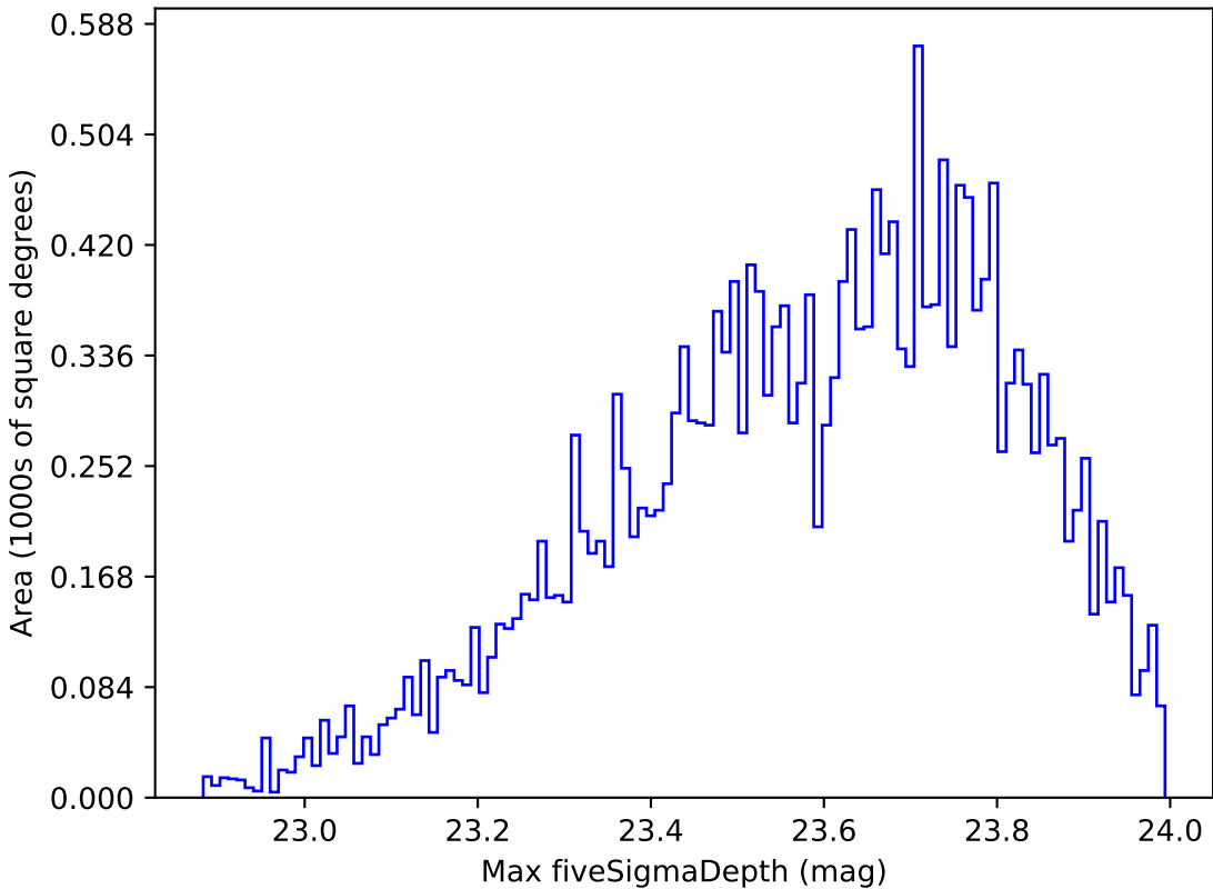
too_elab_r8_d2_gz_v3.4_10yrs Yr 1 u band: Max fiveSigmaDepth
