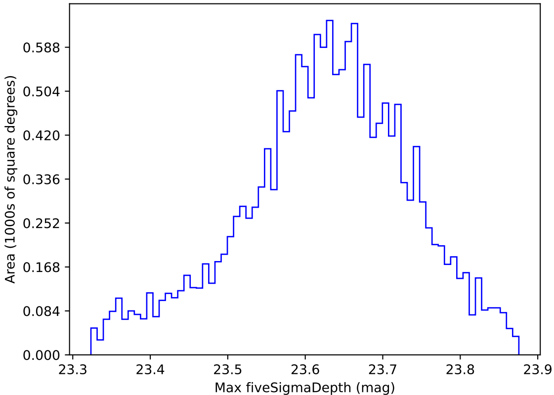
too_elab_r8_d2_gz_v3.4_10yrs WFD z band: Max fiveSigmaDepth
