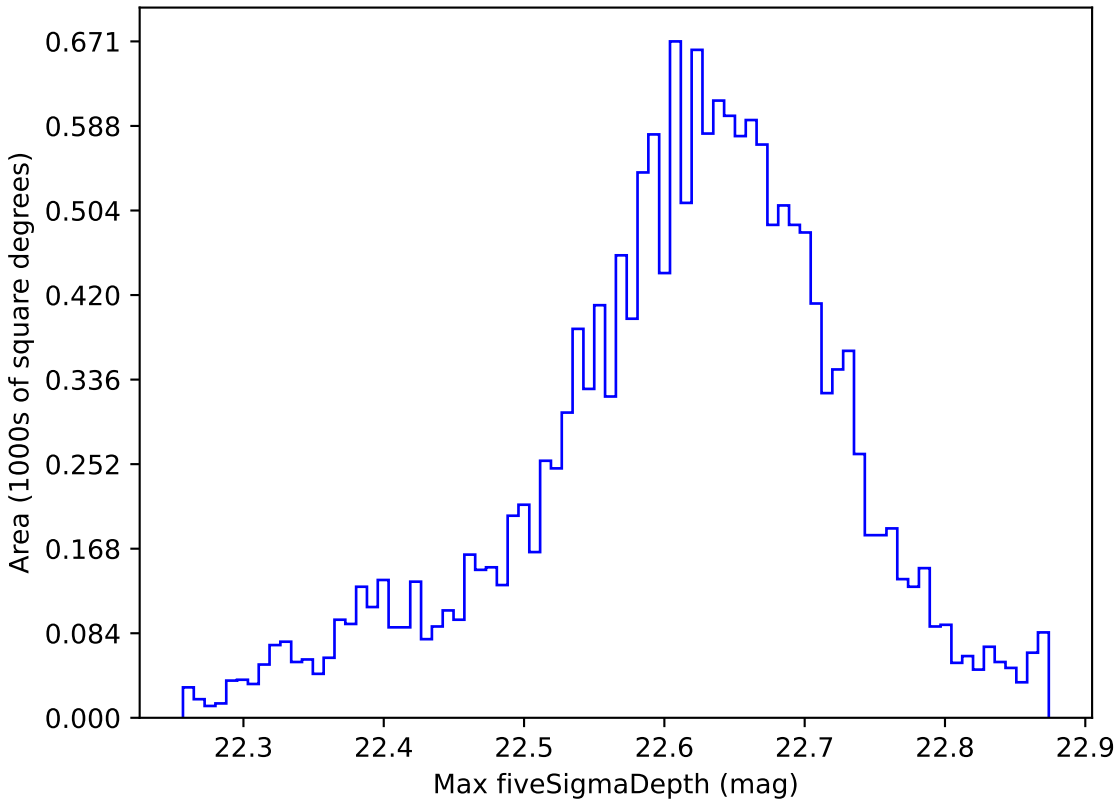
too_elab_r8_d2_gz_v3.4_10yrs WFD y band: Max fiveSigmaDepth
