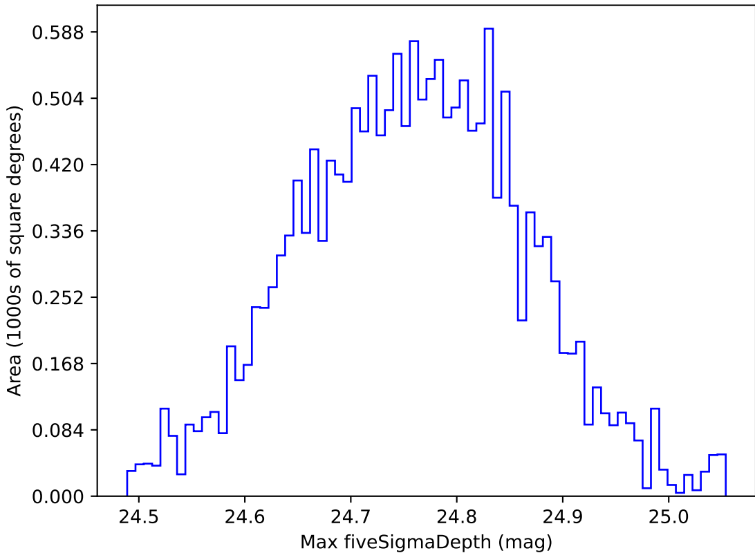
too_elab_r8_d2_gz_v3.4_10yrs WFD r band: Max fiveSigmaDepth
