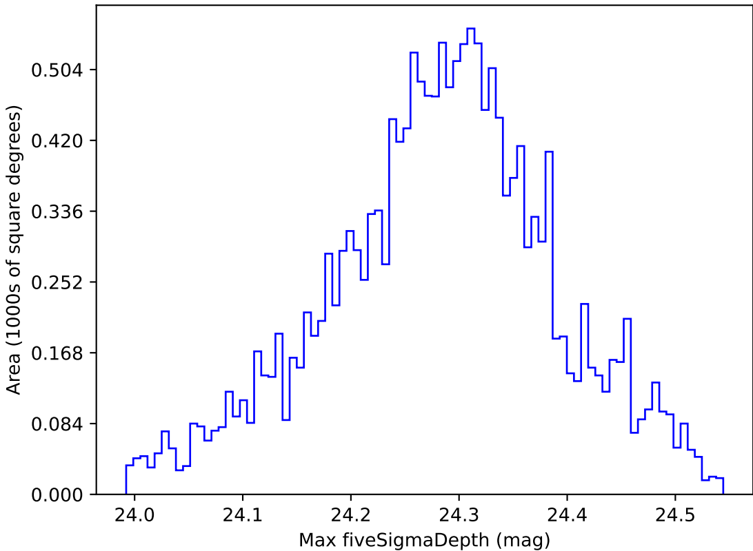
too_elab_r8_d2_gz_v3.4_10yrs WFD i band: Max fiveSigmaDepth
