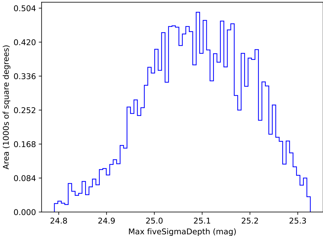
too_elab_r8_d2_gz_v3.4_10yrs WFD g band: Max fiveSigmaDepth
