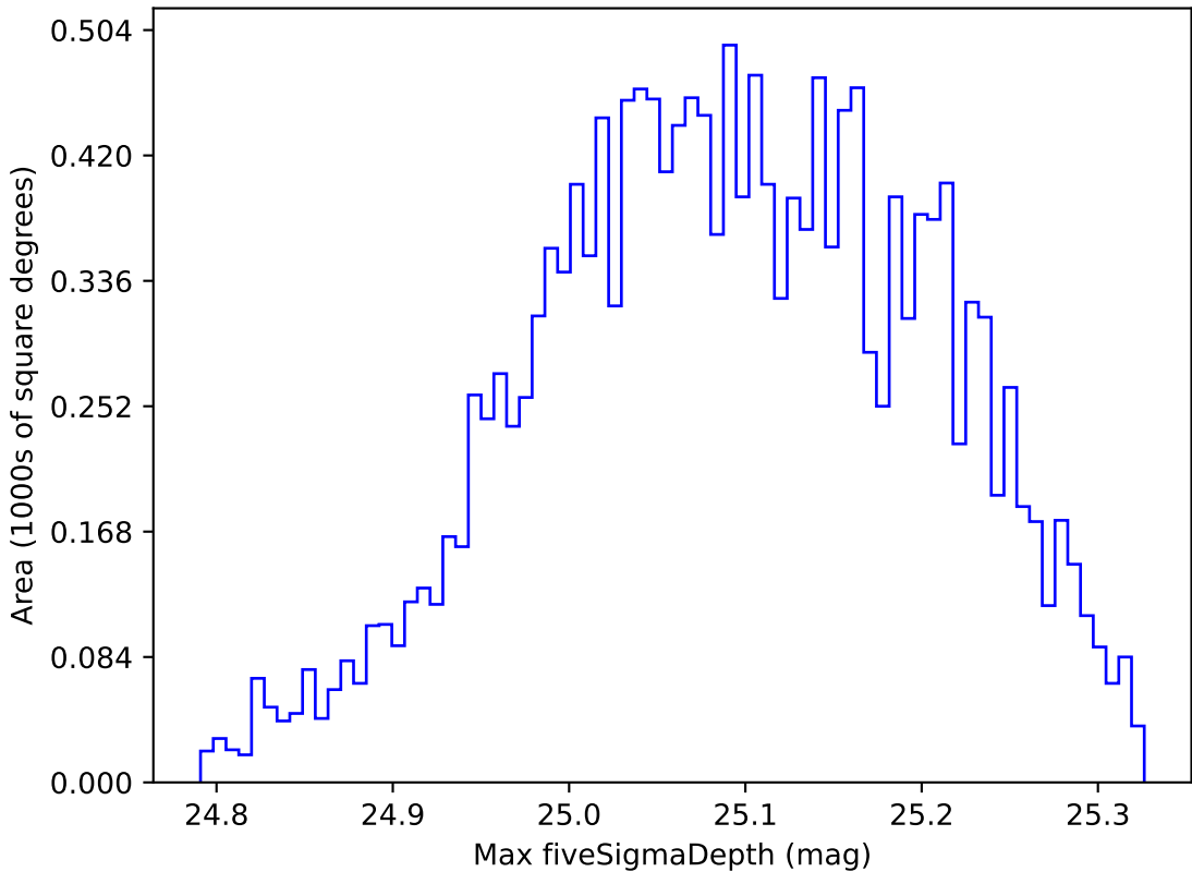
too_elab_r8_d2_gz_v3.4_10yrs WFD all bands: Max fiveSigmaDepth
