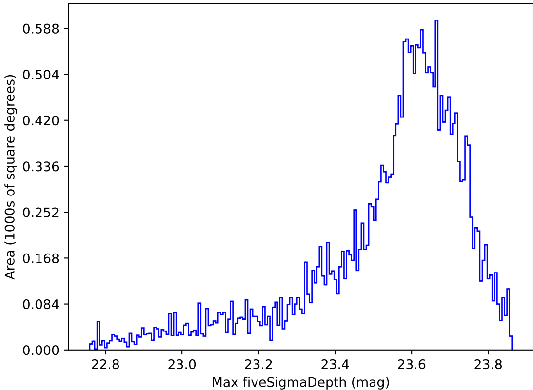
too_elab_r8_d2_gz_v3.4_10yrs All sky z band: Max fiveSigmaDepth
