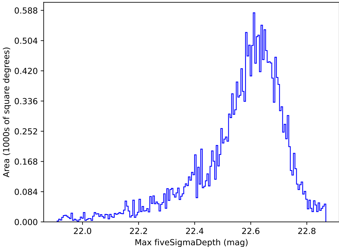
too_elab_r8_d2_gz_v3.4_10yrs All sky y band: Max fiveSigmaDepth
