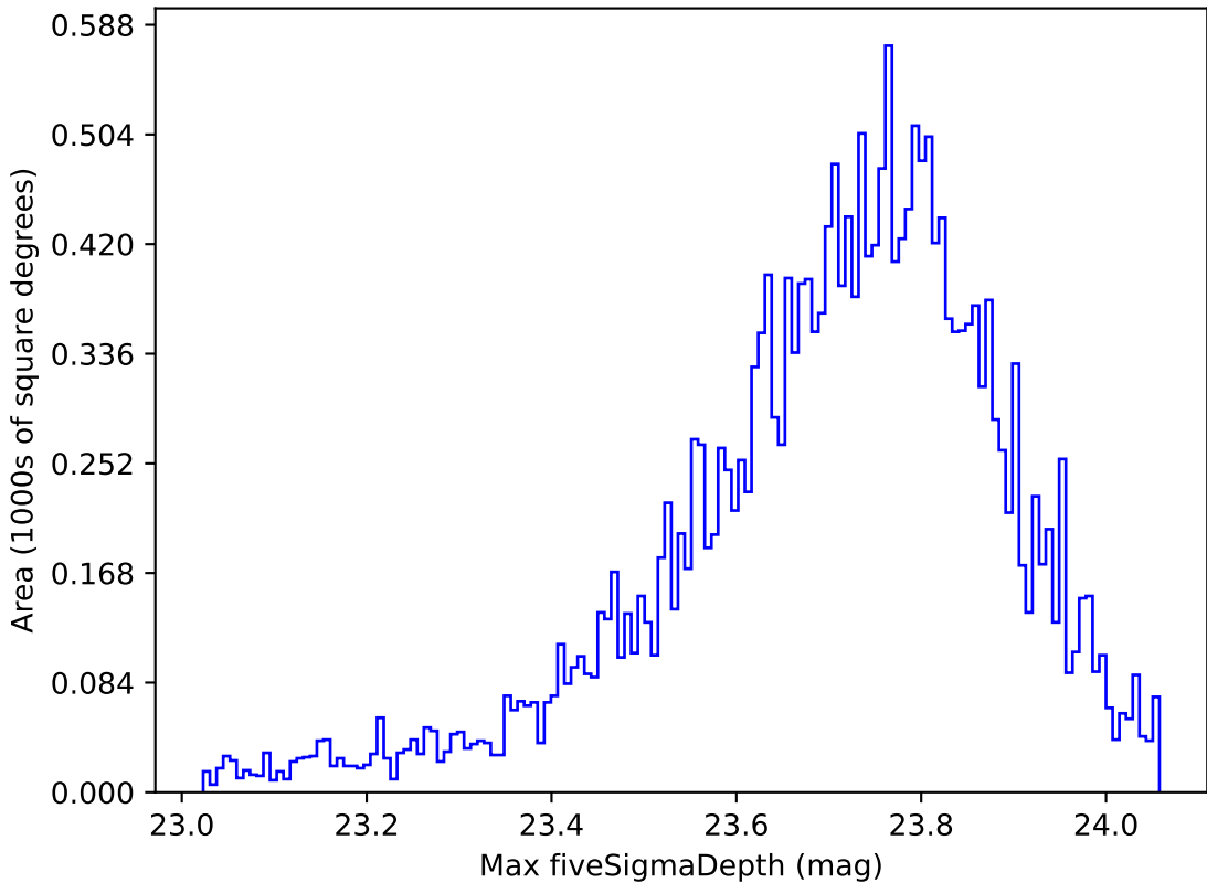
too_elab_r8_d2_gz_v3.4_10yrs All sky u band: Max fiveSigmaDepth
