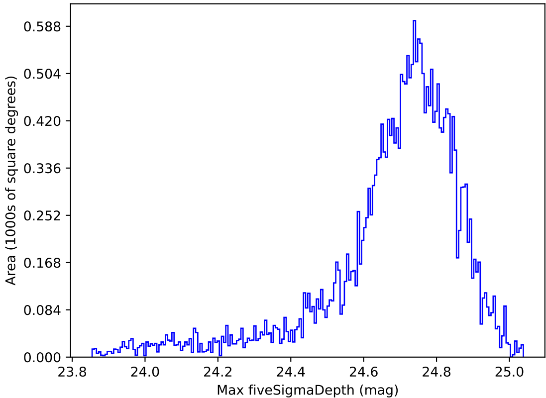
too_elab_r8_d2_gz_v3.4_10yrs All sky r band: Max fiveSigmaDepth
