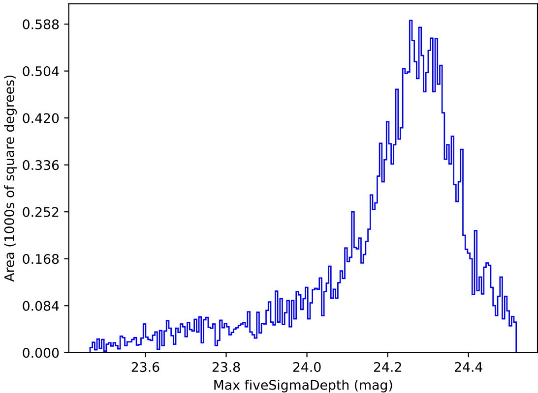
too_elab_r8_d2_gz_v3.4_10yrs All sky i band: Max fiveSigmaDepth
