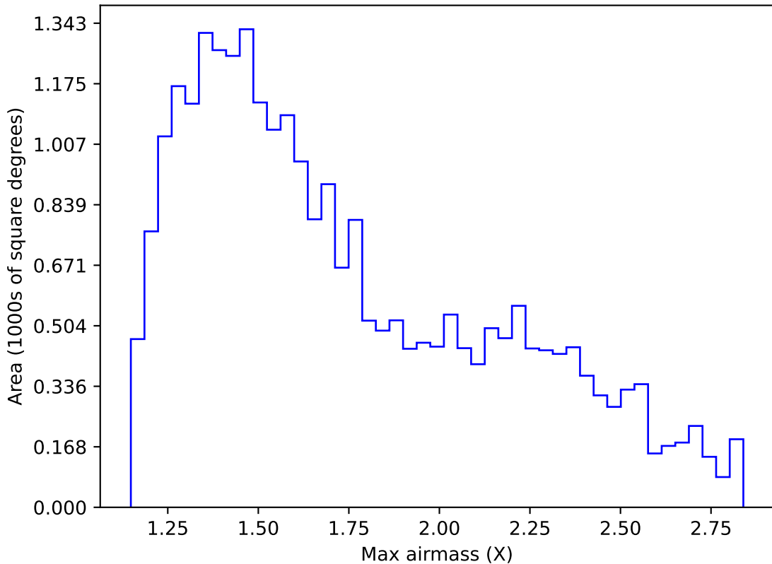
too_elab_r8_d2_gz_v3.4_10yrs Yr 1 z band: Max airmass
