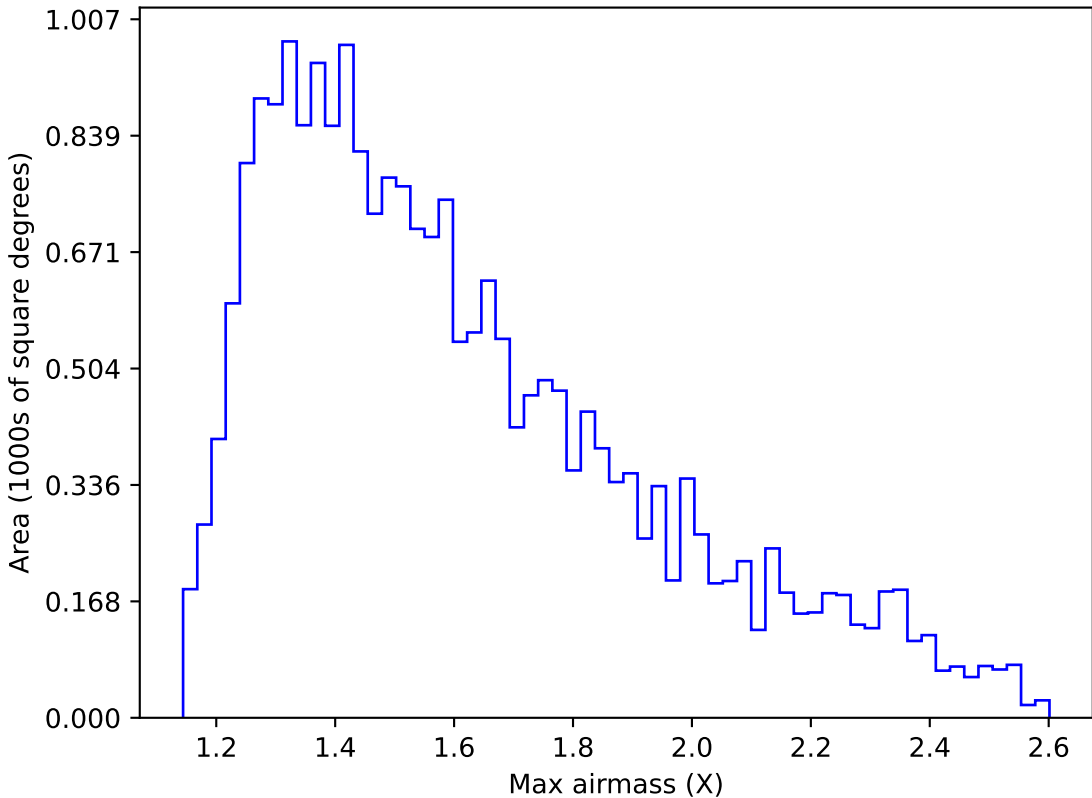
too_elab_r8_d2_gz_v3.4_10yrs Yr 1 y band: Max airmass
