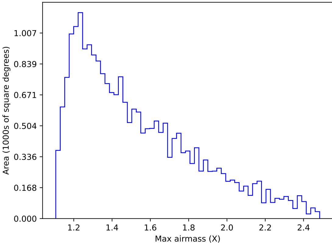
too_elab_r8_d2_gz_v3.4_10yrs Yr 1 u band: Max airmass
