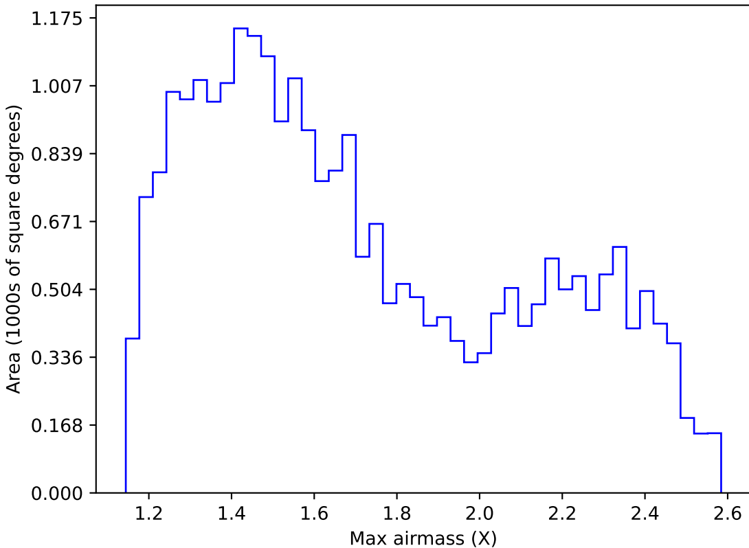
too_elab_r8_d2_gz_v3.4_10yrs Yr 1 r band: Max airmass
